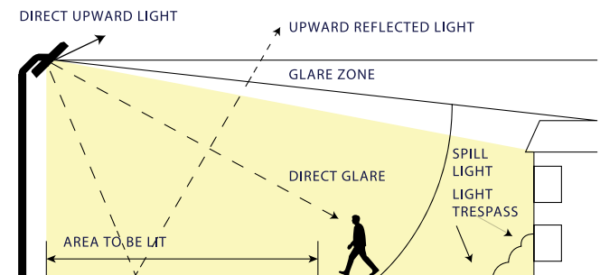
With Symmetric Floodlights
